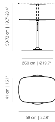
Low table 22.8"x16.1"
